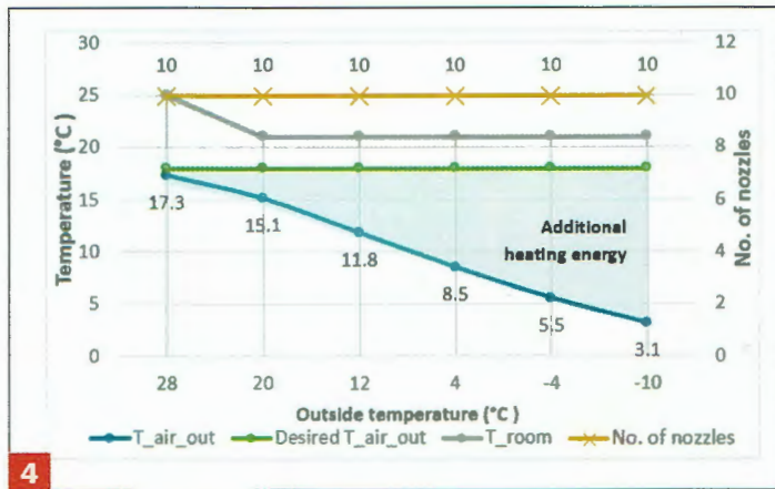
4 Graph showing the number of nozzles and air temperature achieved at different outside temperatures
