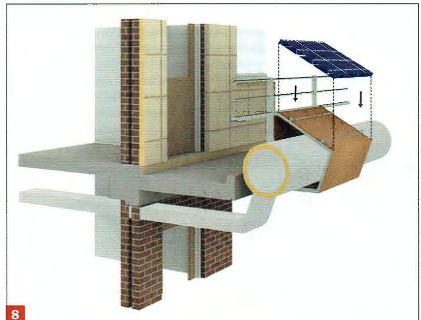
Prefabricated duct cover with solar panel attached to the top
