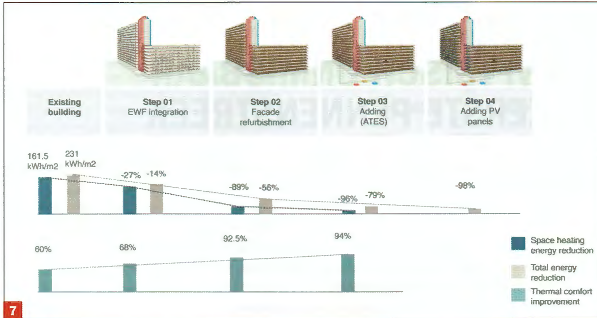
Step-by-step refurbishment strategy with energy savings and comfort performance
