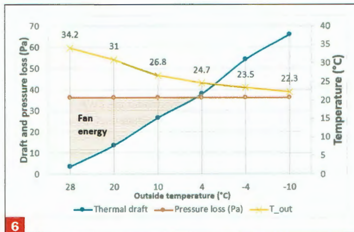
6 Graph showing the pressure loss and thermal draft generated at different outside temperatures
