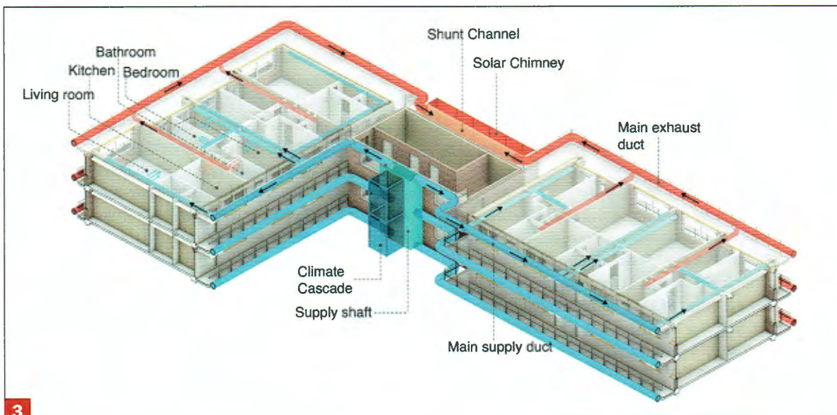
3D section showing the EWF integration and air flow through the building
